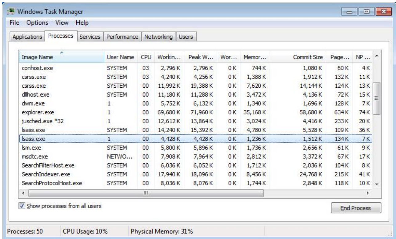
Figure 5. Figure 5: The bot software disguises itself as lsass.exe
