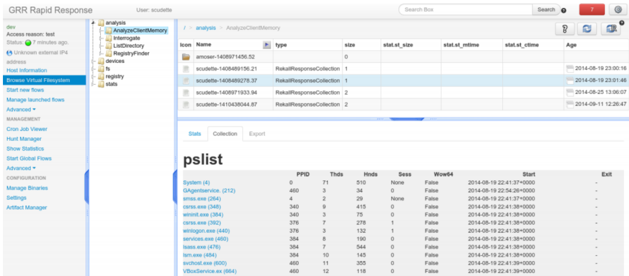
Figure 14. Figure 14: GRR Rapid Response
