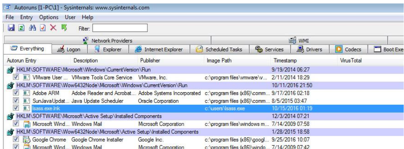
Figure 10. Figure 10: Analyzing startup programs with Autoruns
