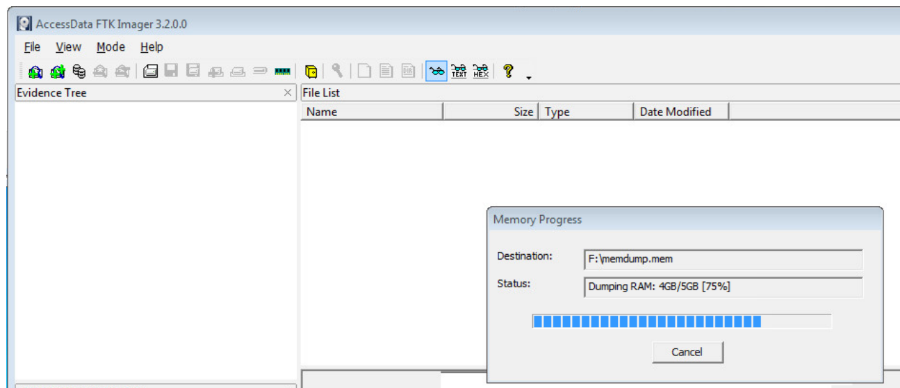
Figure 11. Figure 11: Creating a memory dump of the compromised computer with the FTK Imager utility
